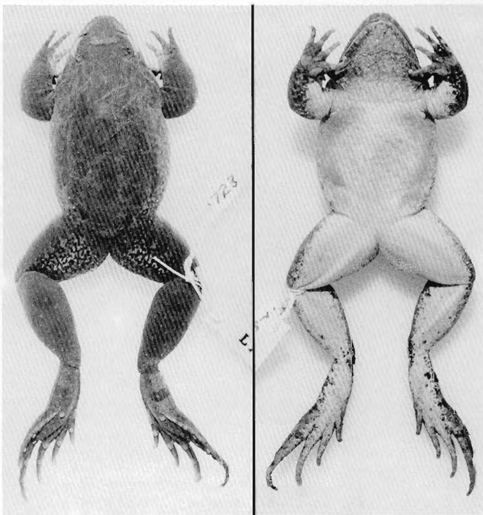
FIGURE 41.—Holotype of Leptodactylus pascoensis , new species.
