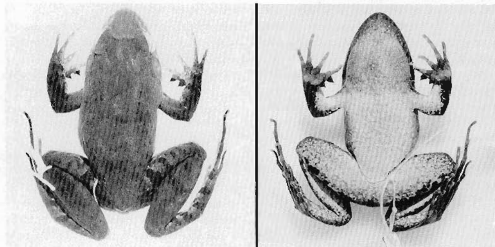
FIGURE 44.—Holotype of Leptodactylus sabanensis , new species.
