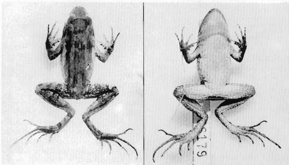
FIGURE 40.—Holotype of Leptodactylus nesiotus , new species.
