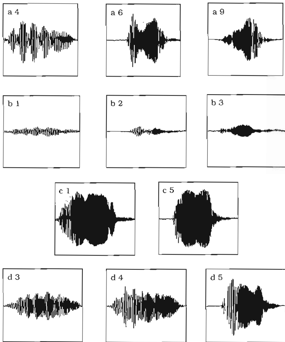
FIGURE 18.—Selected wave forms from audiospectrograms (Figure 17) analyzed from specimen ZUEC 5511 from Cruzeiro do Sul, Acre, Brazil, a member of the Region 4 Anastomotic Belly OTU. All signal lengths = 0.05 s. See legend for Figure 16 for recording data.
