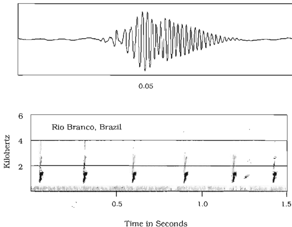
FIGURE 15.—Advertisement calls of Region 4 Light Posterior Belly OTU from Rio Branco, Acre, Brazil, AJC Tape S2, cut 7. Recorded from ZUEC 5639 on 19 Dec 1983, 1915 h, 27°C air, 26°C water, by Adão J. Cardoso. Wave form is of third call shown on audiospectrogram.
